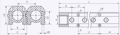
SINGLE DISTRIBUTION MANIFOLD – RED BSPP FEMALE
